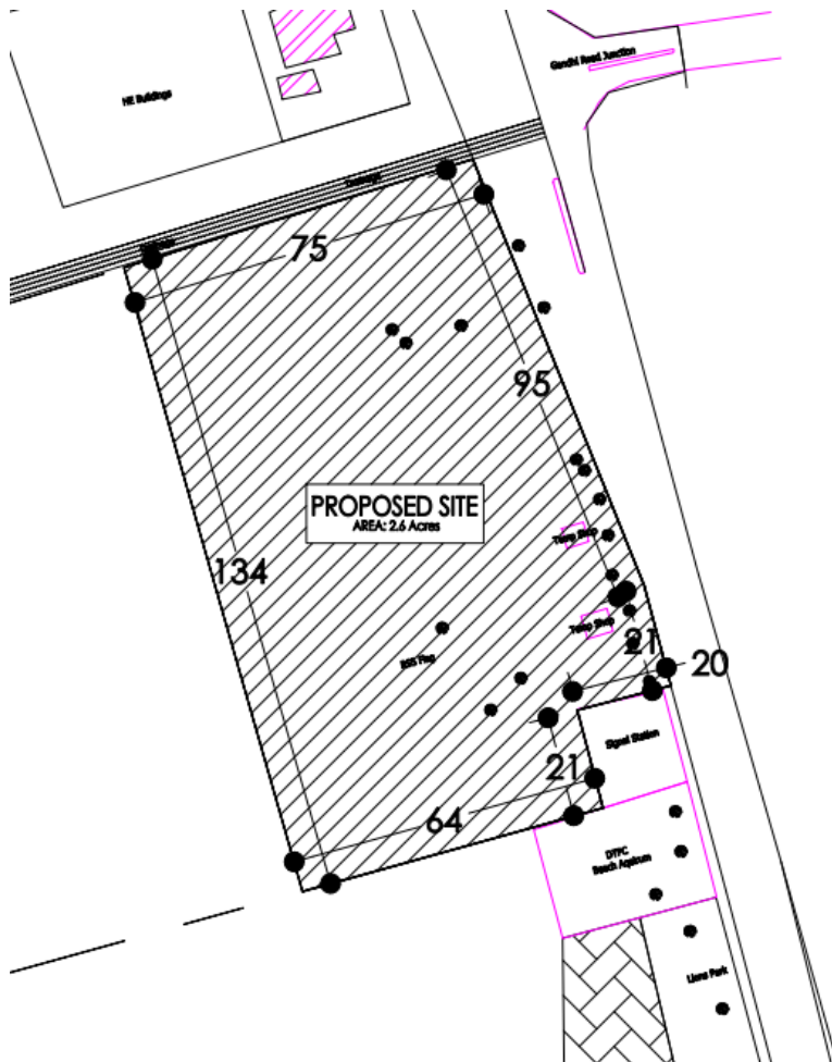
Site Sketch (Dimensions are in Meter)
